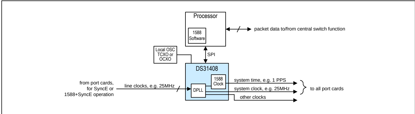
Figure 2-3. Typical Application Example, Frequency and Time Synchronization
