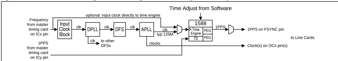
Figure 2-6. 1588 Resource Usage, Slave Timing Card, 1588-Only or 1588+SyncE
