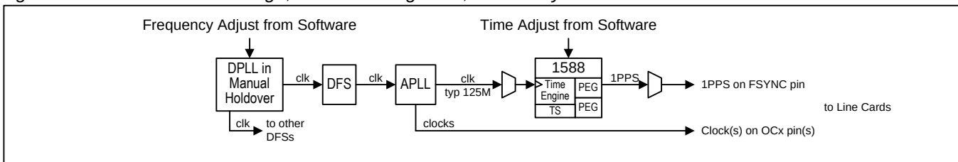
Figure 2-5. 1588 Resource Usage, Master Timing Card, 1588+SyncE Mode
