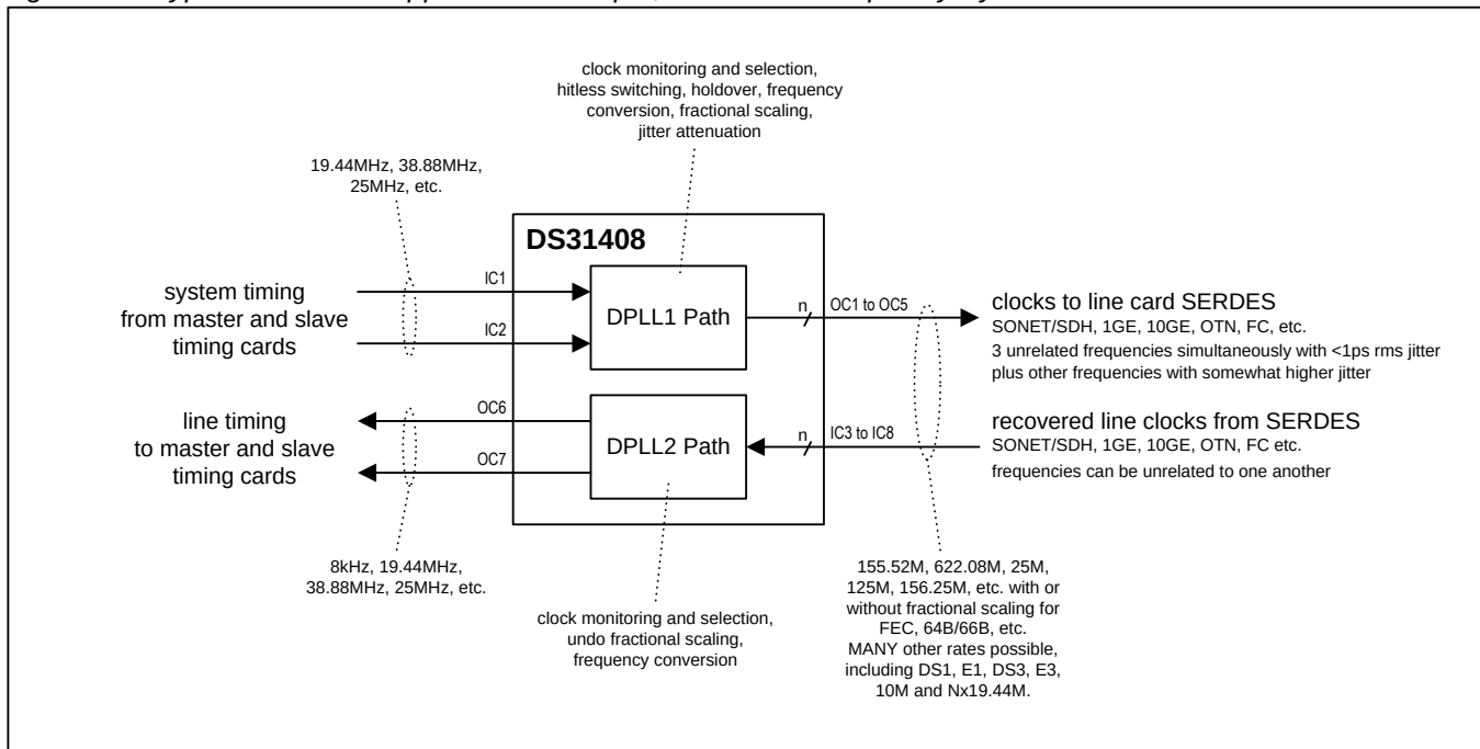
Figure 2-2. Typical Line Card Application Example, Traditional Frequency Synchronization
