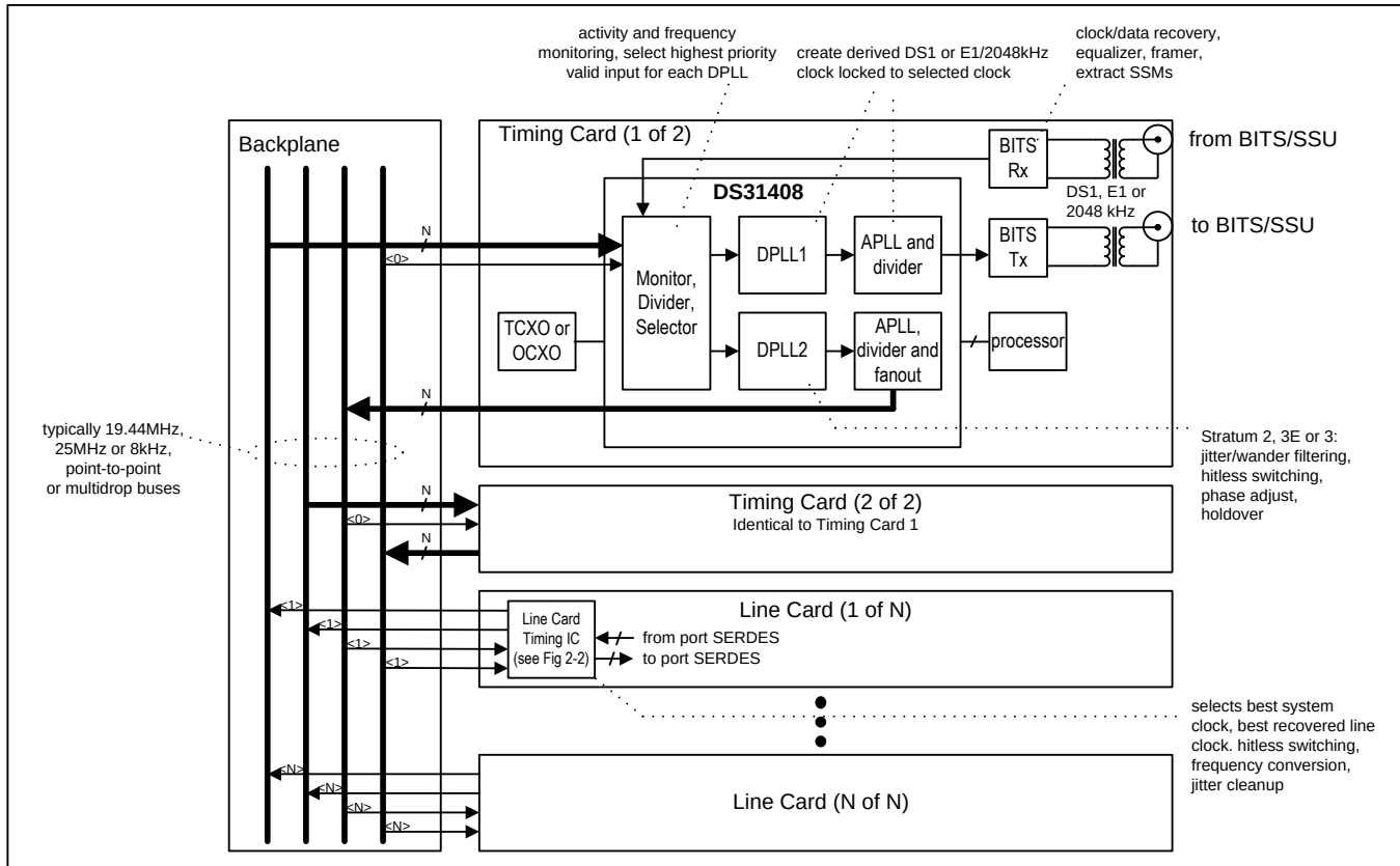
Figure 2-1. Typical Timing Card Application Example
