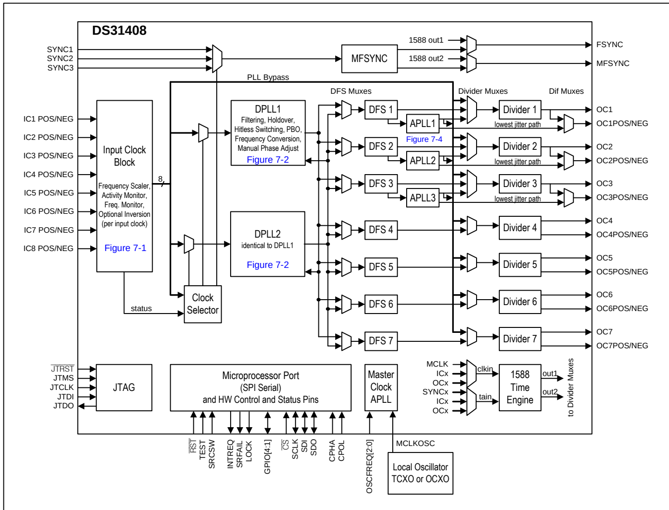
Figure 3-1. DS31408 Block Diagram
