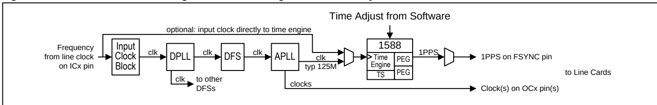
Figure 2-6. 1588 Resource Usage, Slave Timing Card, 1588-Only or 1588+SyncE
