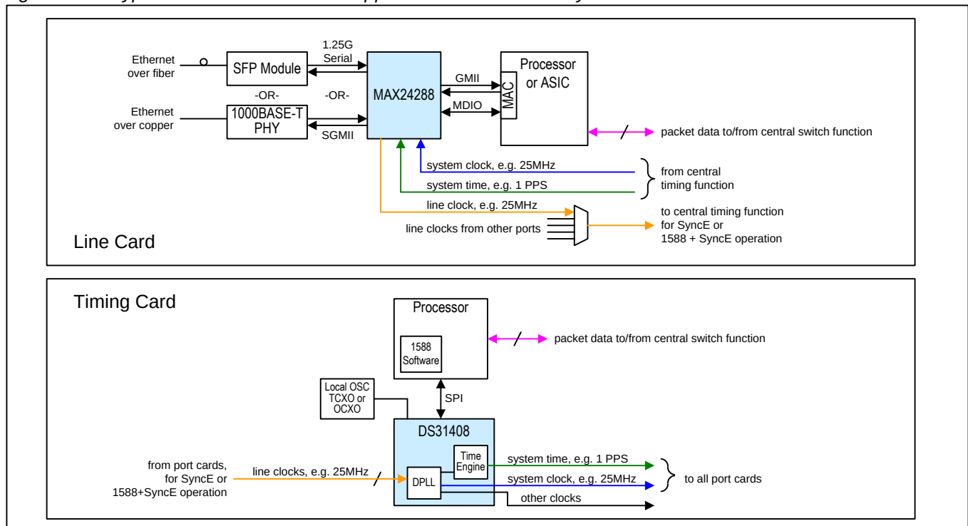
Figure 7-13. Typical DS31408 IEEE1588 Application in a Telecom System
