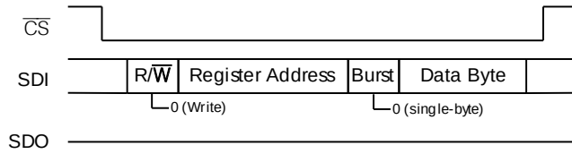
Figure 7-12. SPI Bus Transactions
